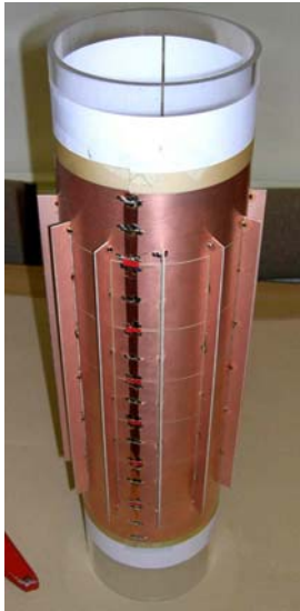
Internal view of sliding sensor showing radial screens
