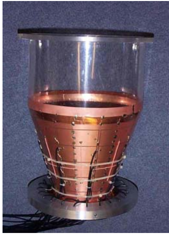
Conical sensor internal view
